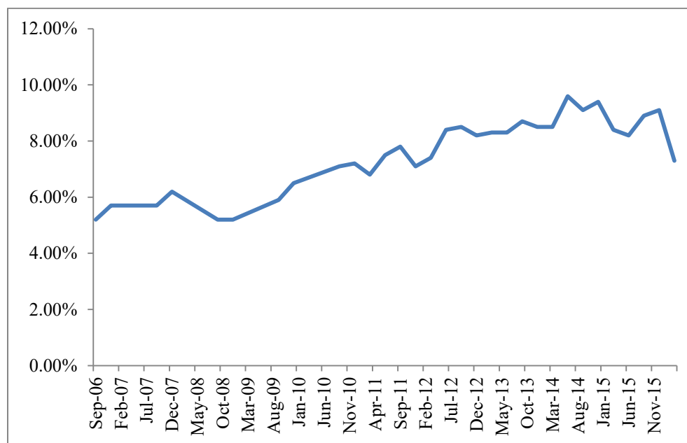
Figure 5: NPL Ratio
